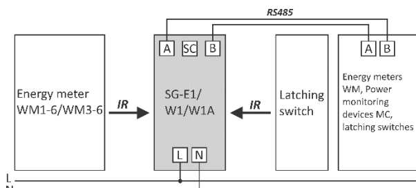
Figure 1: Diagram of various devices wired to SG.
