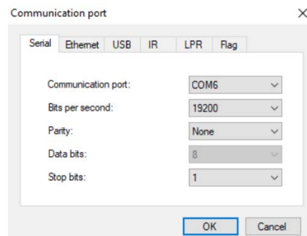
Figure 9: Communication port window
